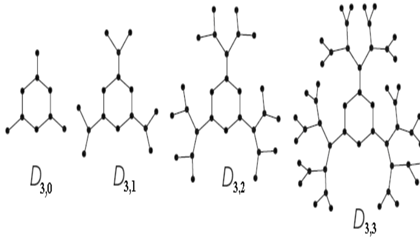
Figure 2. The graph of hexagonal cored dendrimers with generation numbers 0, 1, 2, 3.
