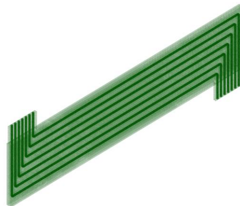
Fig. 3. 3-fluid LAMEE grid system.
