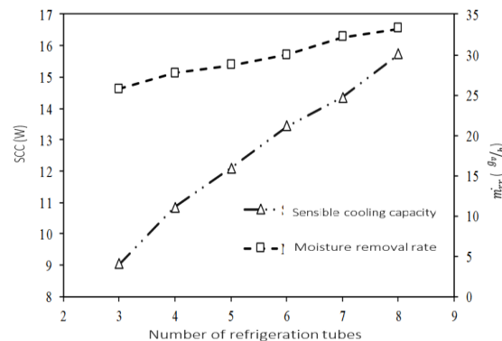
Fig. 6. The effect of the number of cooling tubes on the sensible cooling capacity and moisture removal rate.
