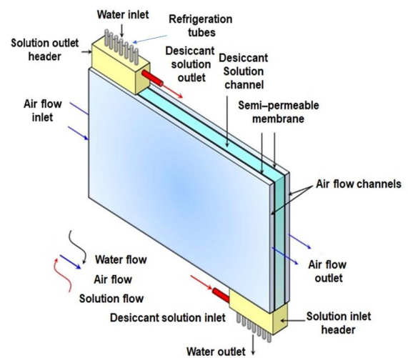
Fig.1. Diagram for the 3-fluid LAMEE[1].
