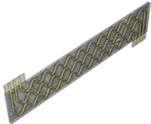
Fig. 11. 3-fluid LAMEE with three wavy refrigeration tubes.
