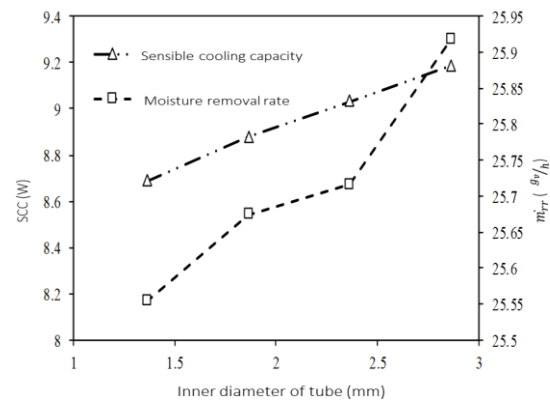
Fig. 9. Variations of the sensible cooling capacity and moisture removal rate with the inner diameter of the refrigeration tubes.
