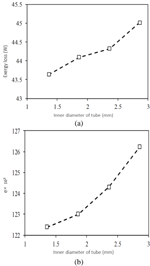
Fig. 10. The effect of the diameter of the refrigeration tubes on: (a) exergy loss, and (b) dimensionless exergy loss.
