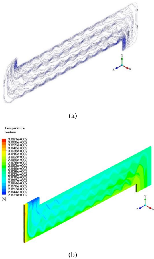
Fig. 14. (a) Streamlines of the dehumidifier fluid, (b) temperature contour of the dehumidifier fluid stream.
