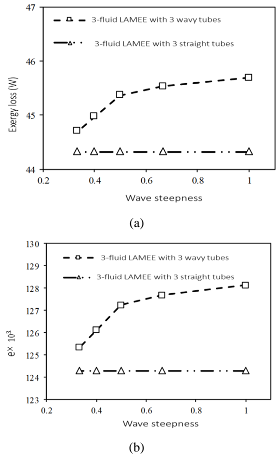
Fig. 15. The effect of the wavy refrigeration tubes on: (a) exergy loss, and (b) dimensionless exergy loss.
