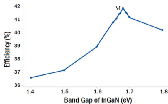
Fig. 5: The effect of the band gap of InGaN on efficiency.
