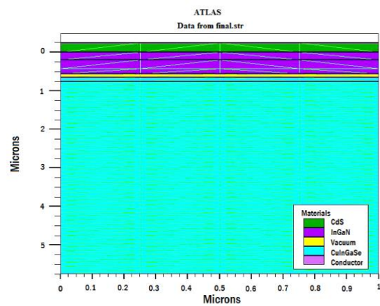
Fig. 2: Meshing structure.
