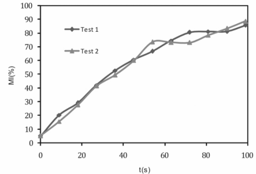
Fig. 11. Repeatability of experiments ( L = \frac{\pi}{3}R_b , \omega_{ave} = 15(Re \approx 20) and \Delta\omega = 10 rpm for both tests).
