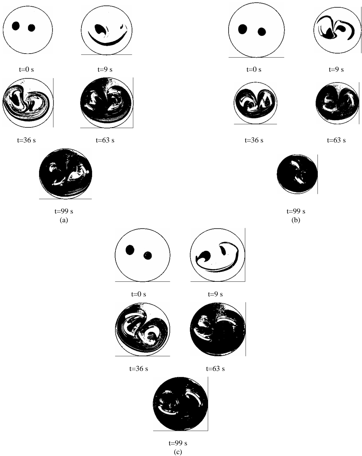
Fig. 7. Deformation of blob for various values of the length of blades; (a) L = \frac{\pi}{6}R_b , (b) L = \frac{\pi}{3}R_b , (c) L = \frac{\pi}{2}R_b ( \omega_{ave} = 15 \text{ rpm} ( Re \approx 20 ) and \Delta\omega = 10 \text{ rpm} for all cases).
