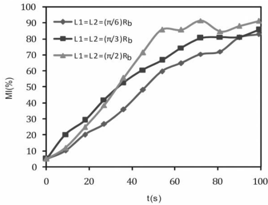
Fig. 8. Effect of the length of blades on mixing index ( \omega_{ave} = 15 \text{ rpm} and \Delta\omega = 10 \text{ rpm} for all cases)
