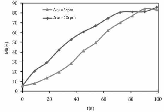
Fig. 9. Effect of rotational speed amplitude of blades on mixing index ( L = \frac{\pi}{3}R_b and \omega_{ave} = 15 \text{ rpm} ( Re \approx 20 ) for both case
