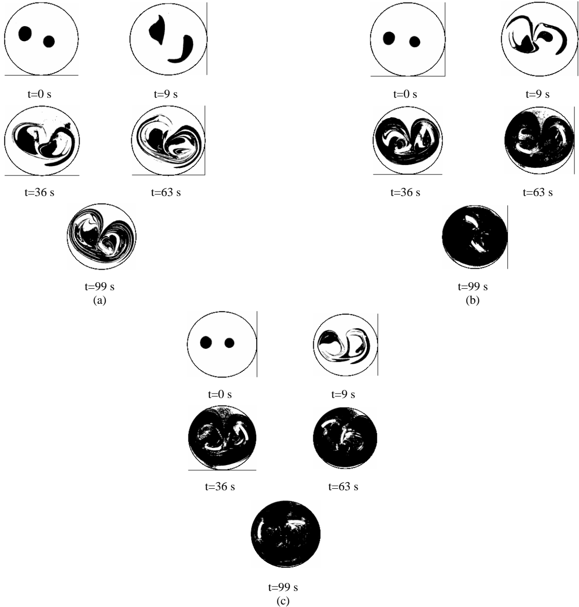
Fig. 5. Deformation of blob at various average rotational speed; (a) \omega_{ave} = 7.5 rpm ( Re \approx 5 ) ( Re ), (b) \omega_{ave} = 15 rpm ( Re \approx 10 ), and (c) \omega_{ave} = 30 rpm ( Re \approx 20 ) ( L = \frac{\pi}{3} R_b and \Delta\omega = 10 rpm for all cases).
