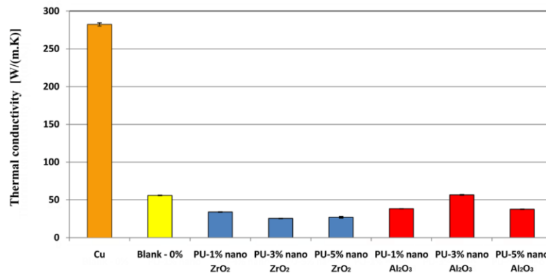
Fig. 5. Standard deviation of thermal conductivity of nanocomposite coating on copper plate with 0, 1,3 and 5% of zirconium oxide and aluminum oxide nanoparticles.
