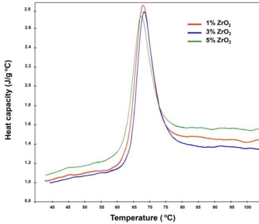
Fig. 3. Specific heat capacity of urethane nanocomposites containing 1, 3, and 5-wt% nanozirconium oxide.
