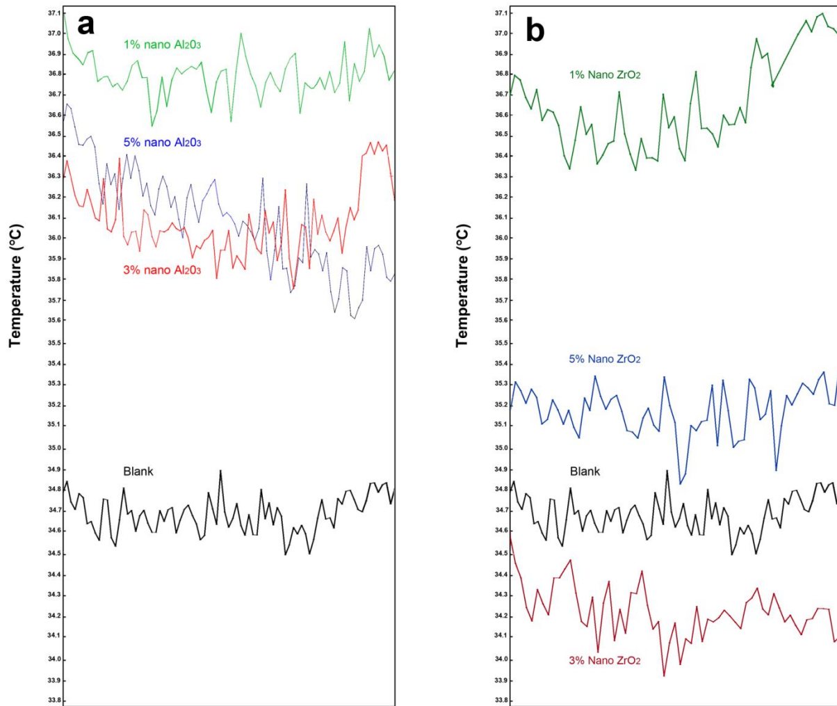
Fig. 6. Thermography results of nanocomposite coating on copper plate. a) Samples with 0, 1, 3 and 5% of aluminum oxide nanoparticles and b) Samples with 0, 1, 3 and 5% of zirconium oxide nanoparticles.
