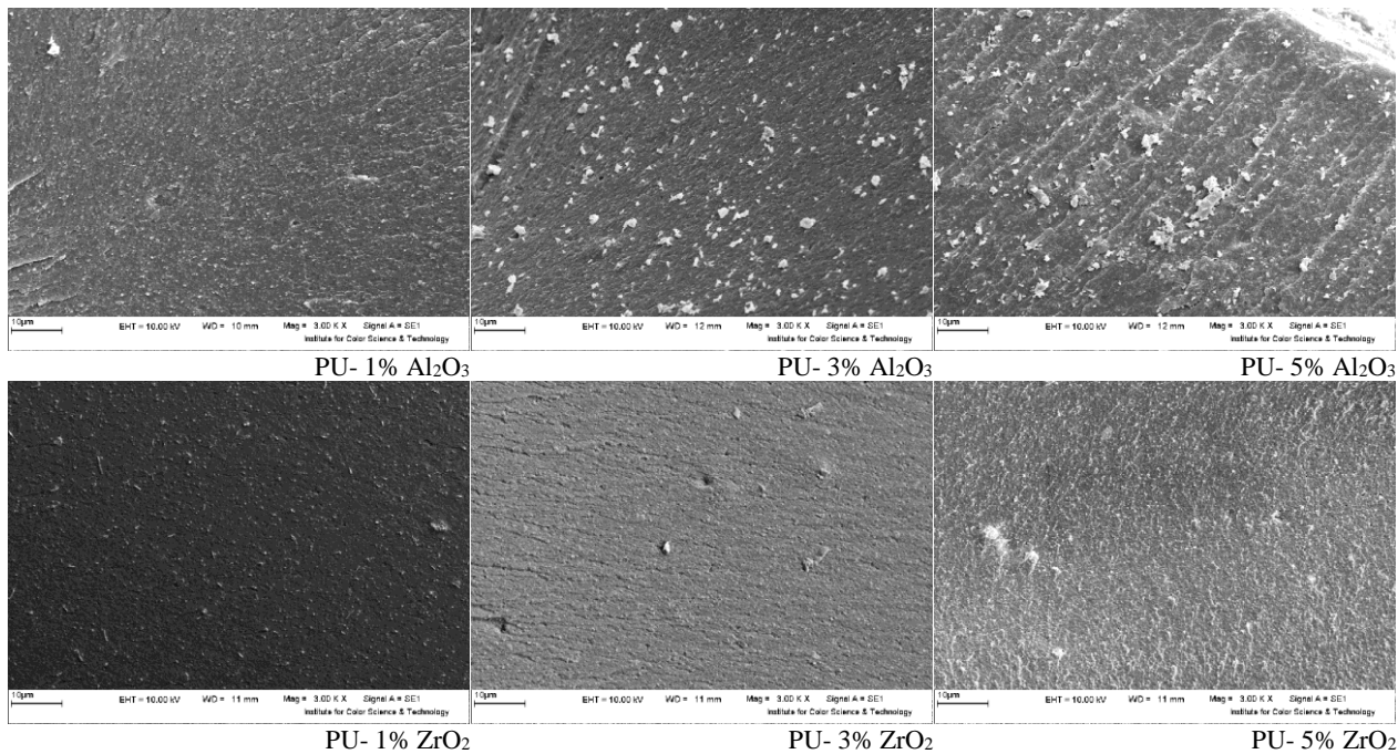
Fig. 1. SEM images of urethane nanocomposites with various nanoparticles.
