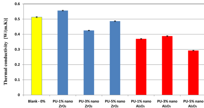
Fig. 4. Standard deviation of thermal conductivity of nanocomposite coatings with 0, 1, 3 and 5% of zirconium oxide and aluminum oxide nanoparticles.
