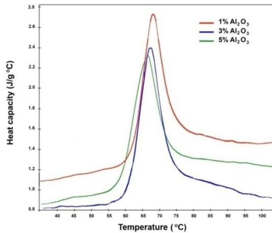
Fig. 2. Specific heat capacity of urethane nanocomposites containing 1, 3, and 5wt% nano aluminum oxide.
