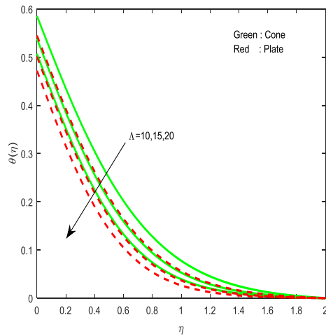
Fig. 41. Variations of the buoyancy parameter \Lambda on the dimensionless temperature.
