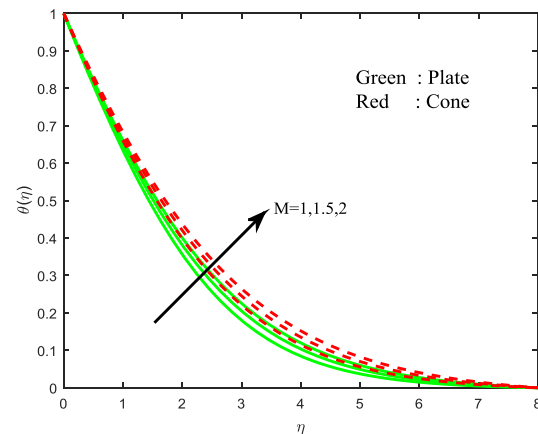
Fig. 3. Temperature profiles for different values of magnetic field parameter.
