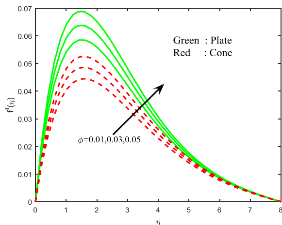
Fig. 4. Velocity profiles for different values of the nano particle volume fraction.
