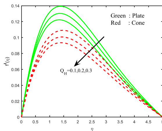
Fig. 8. Velocity profiles for different values of heat source parameter.
