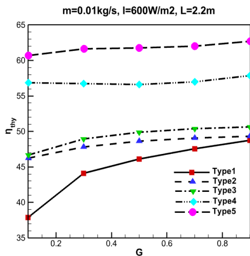
Fig. 7. Variation of thermo-hydraulic efficiency against the reflux ratio.
