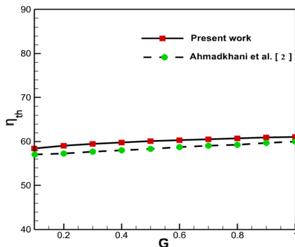
Fig. 3. Comparison of the thermal efficiencies of the Type 2 air heater in the present study with the research conducted by Ahmadvhani et al. [2].
