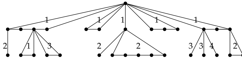
Figure 4. A 4-dimensional plane Husimi graph on 30 vertices.
