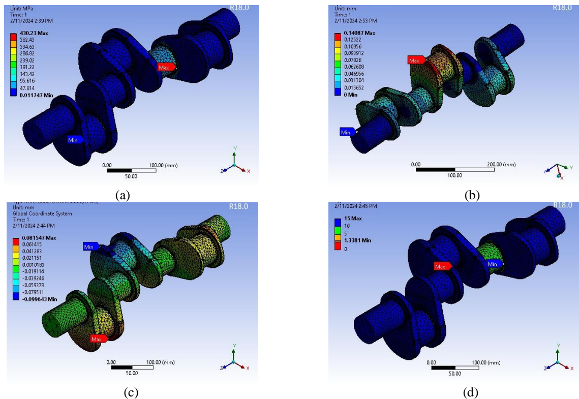
Fig. 3. Original model solutions: (a) Equivalent von-mises stress distribution, (b) Total deformation distribution, (c) Axial deformation distribution, and (d) Safety factor values distribution.
