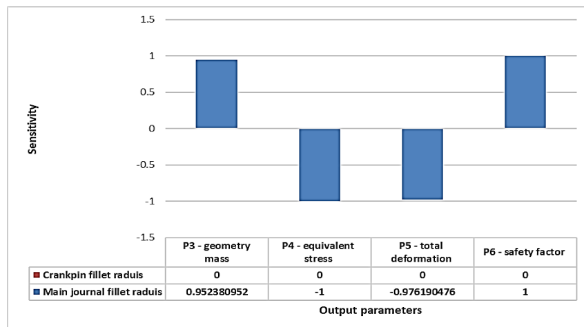
Fig. 5. Sensitivity analysis chart for output optimization parameters.
