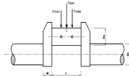
Fig. 1. Applied forces acting on v6-crankpin.
