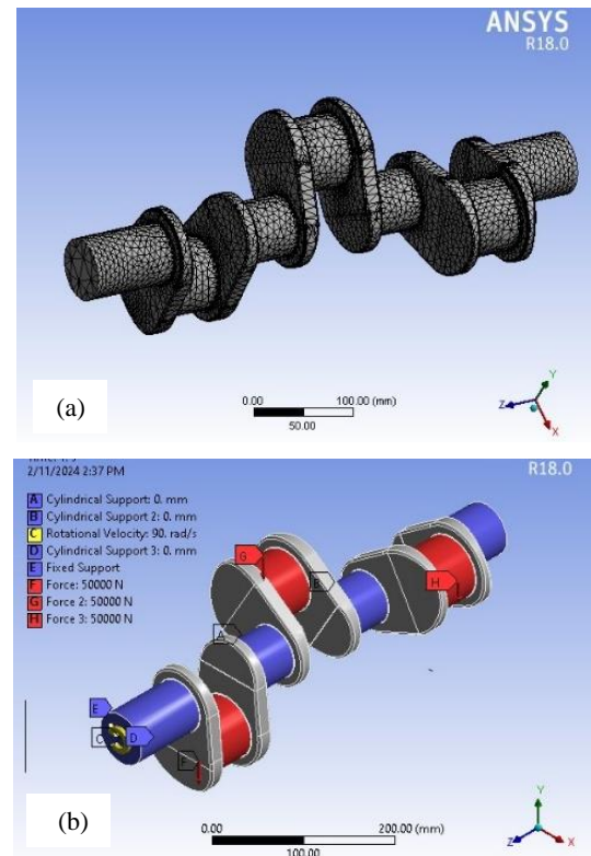
Fig. 2. (a) FEA model and (b) boundary conditions.
