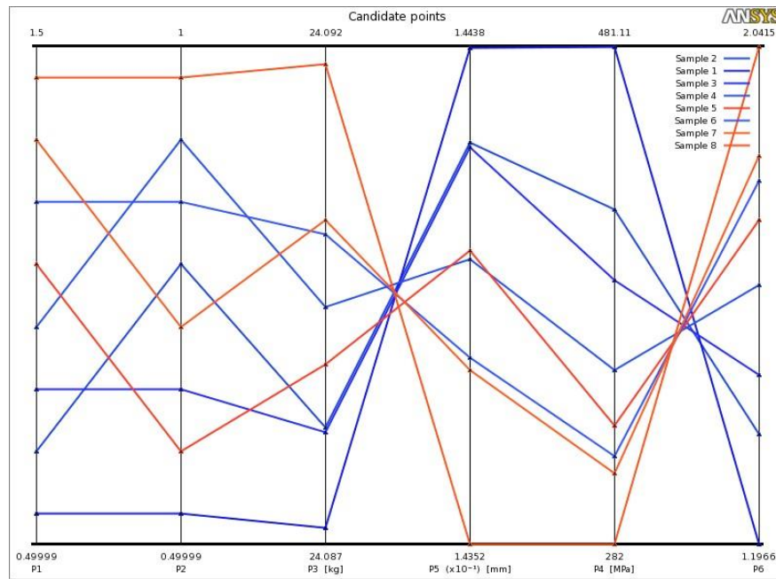
Fig. 4. Sample design points chart.
