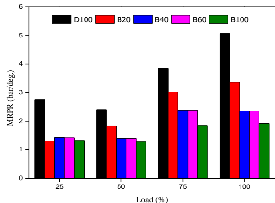
Fig. 9. MRPR versus engine load.
