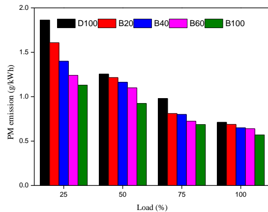
Fig. 13. PM emission versus engine load.
