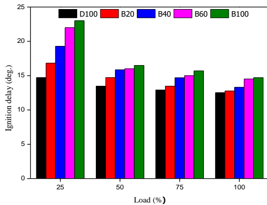
Fig. 7. Ignition delay verses engine load.
